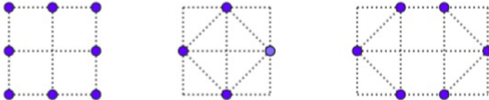
Figure 1. MSC_4 , MSC'_8 , and MSC_8 .
