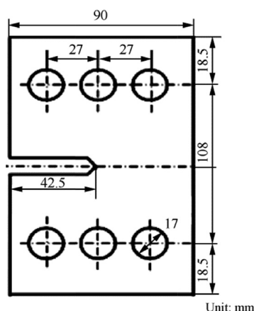
Fig. 6 Dimensions of a CTS specimen. 21,35
