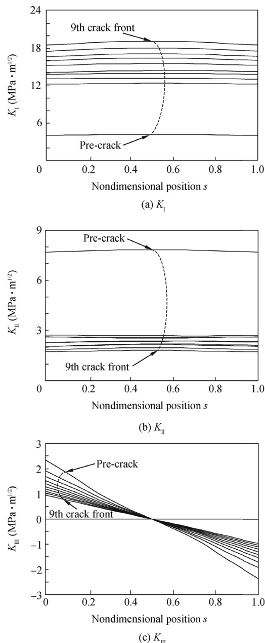
Fig. 11 Distributions of mixed mode SIFs along the crack front for each crack propagation step under 75° loading angle.
