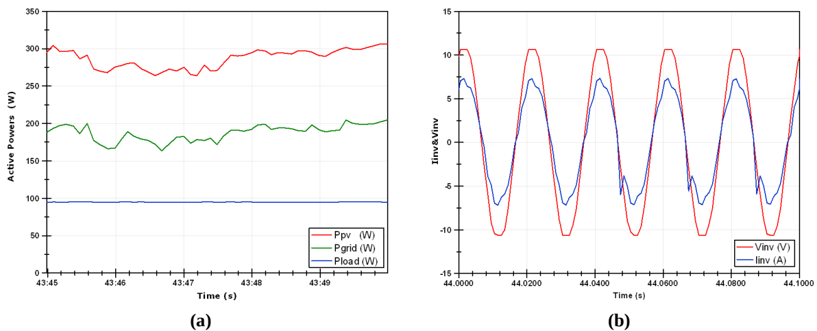
Figure 6. (a) The active power changes of the PV system, (b) The waveforms of the current and voltage of the inverter
