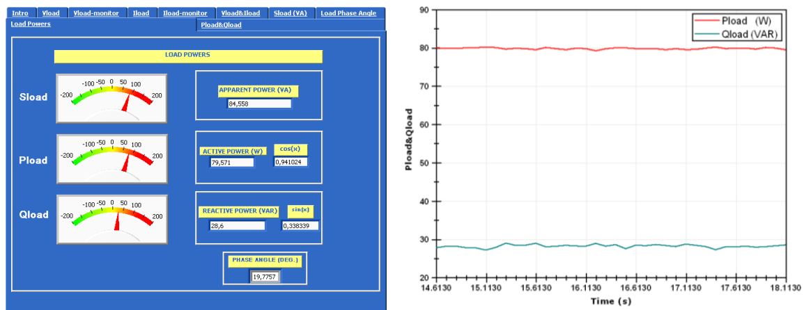
Figure 7. (a) The power and phase angle of the inverter, (b) The load power in real-time
