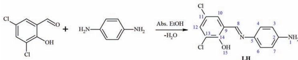
Scheme 1. Preparation of the ligand.
